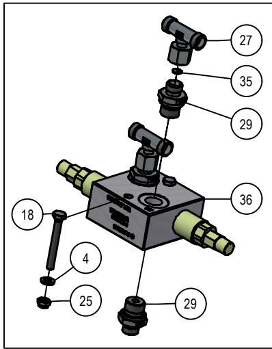
Detail A
